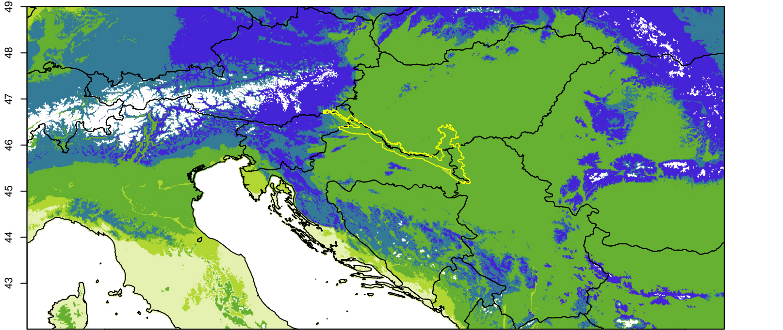
RCP8.5 2081-00
