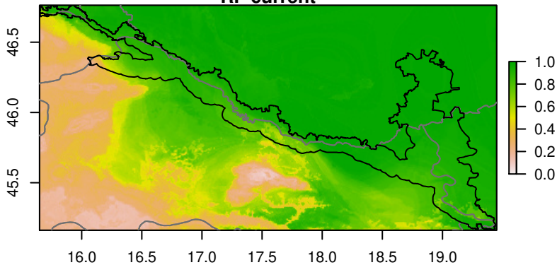
RF current
