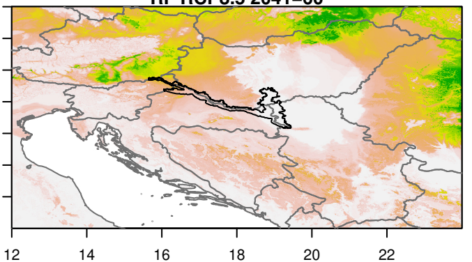
RF RCP8.5 2041–60
