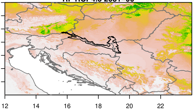
RF RCP4.5 2081–00
