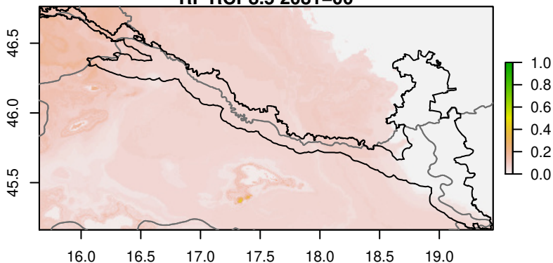
RF RCP8.5 2081–00
