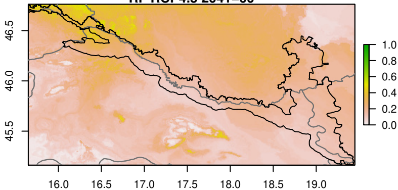
RF RCP4.5 2041–60
