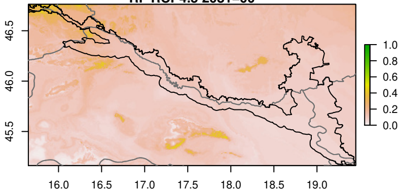
RF RCP4.5 2081–00
