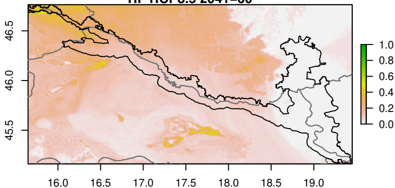
RF RCP8.5 2041–60
