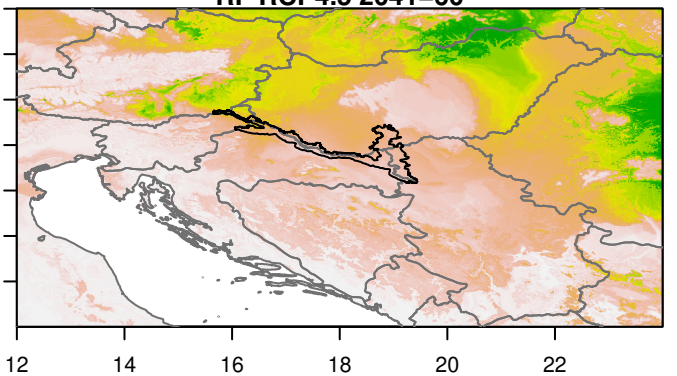
RF RCP4.5 2041–60
