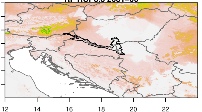
RF RCP8.5 2081–00
