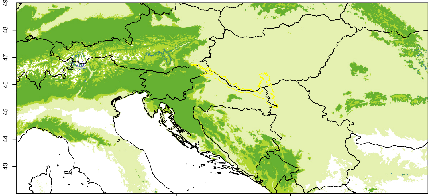
RCP8.5 2081-00
