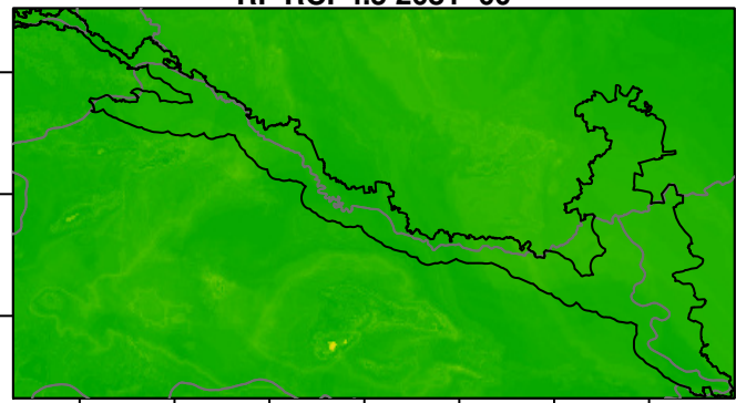
RF RCP4.5 2081–00
