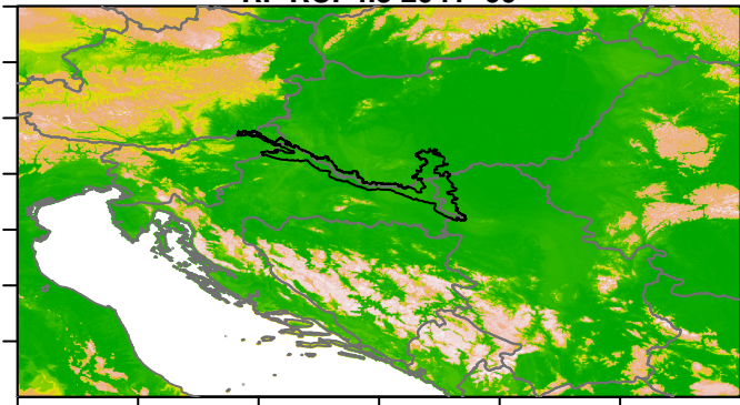
RF RCP4.5 2041–60
