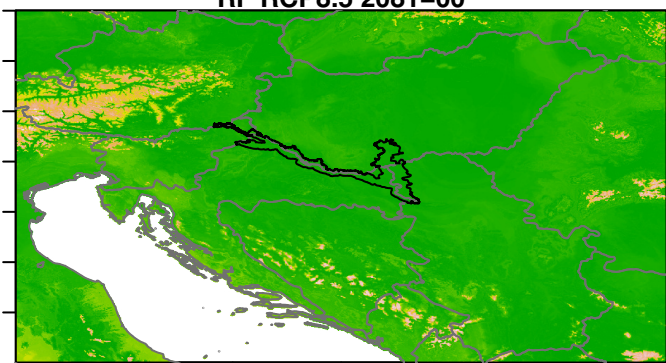
RF RCP8.5 2081–00
