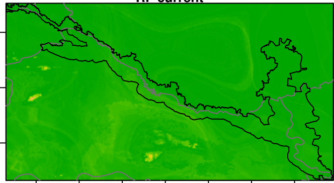
RF current
