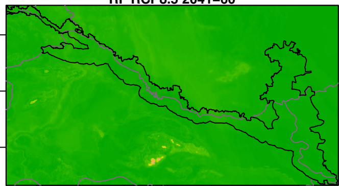
RF RCP8.5 2041–60
