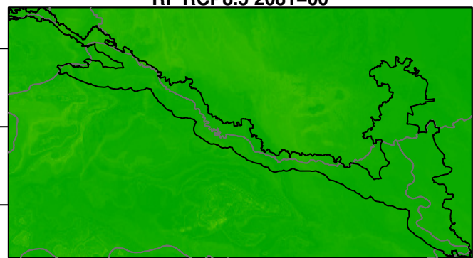
RF RCP8.5 2081–00
