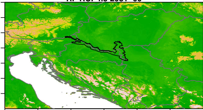
RF RCP4.5 2081–00
