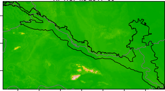
RF RCP4.5 2041–60
