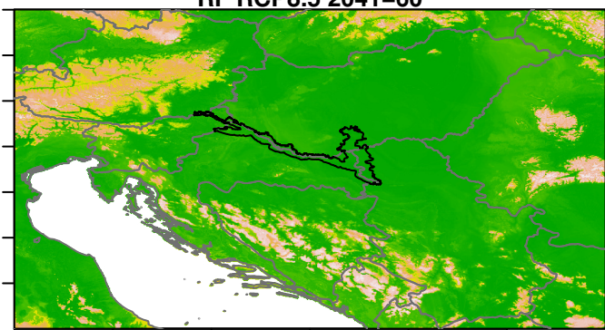
RF RCP8.5 2041–60
