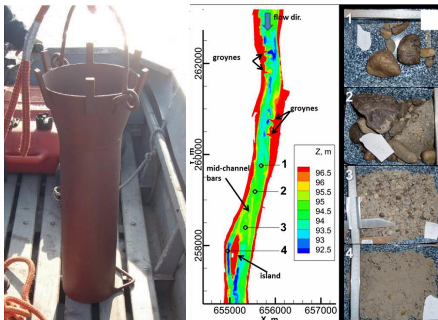
Figure 3.15: Left: Grab sampler (Source: Nikolett Tókési) and an example of locations of bed material sampling and photos of related dried samples (right)
