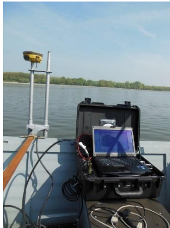
Figure 3.4: EcoTrac GPS receiver and a connected single beam echo sounder used for riverbed topography measurements in Hungary (Source: Debóra Varga-Lehofer)
