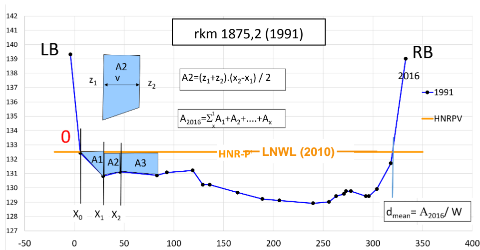
Figure 4.8: Calculation of the cross-sectional area between the riverbed and the low-flow water level (2016)
