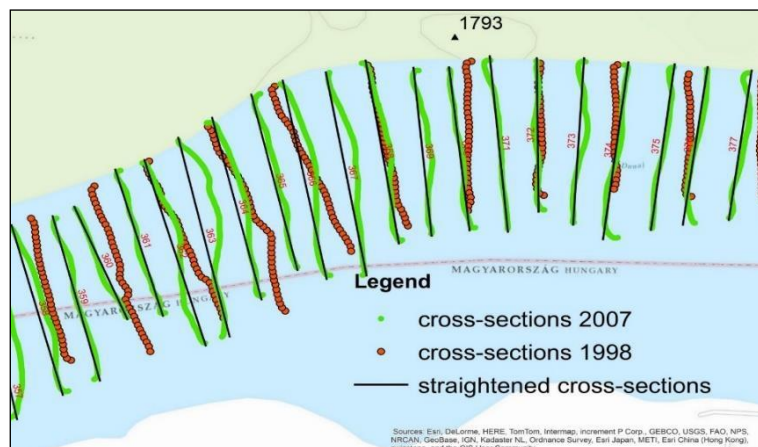
Figure 4.7: Examples of cross-sections straightened for the differences
