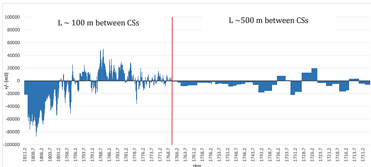
Figure 4.10: Riverbed changes ( m^3 ) assessed in the Danube's SK-HU section (rkm 1,810–rkm 1,709) in Period III (1991/2016)
